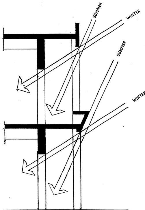
Fig. (5). Optimization studies show that the introduction of the permanent solarium overhangs, even when effectively designed, result to a reduction of heating savings by 8%.
