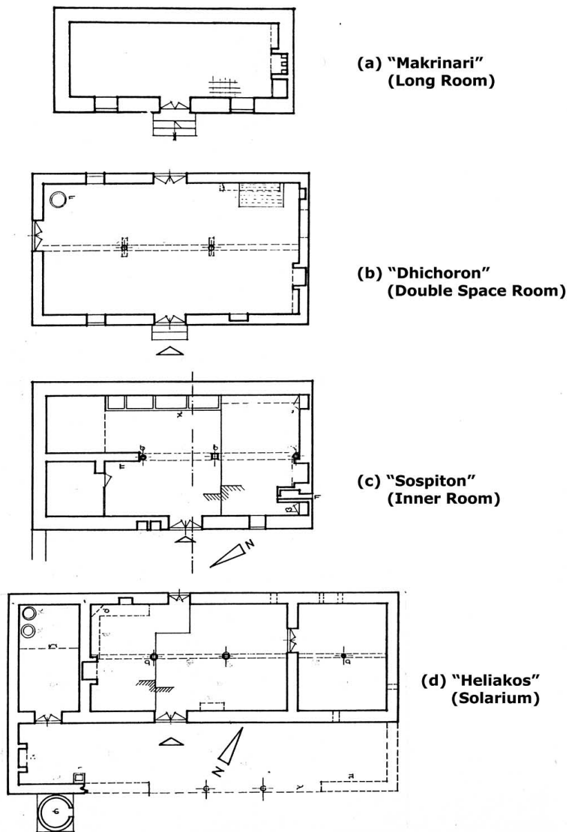
Fig. (2). The evolution of the Cyprus house. An archetypal form of a single, long, rectangular roomed building is revealed as the simplest basic shelter of the Cypriots.
