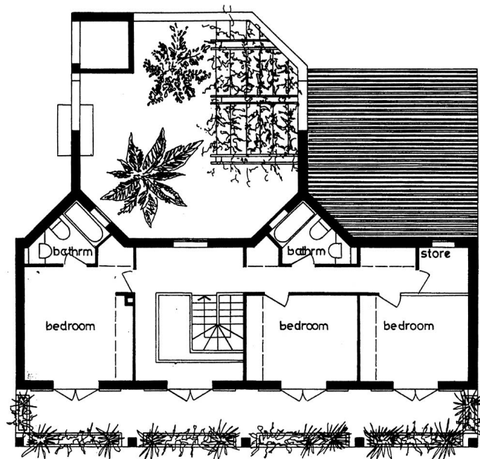
Fig. (4). The more complex courtyard houses save more energy in the house than simpler forms.
