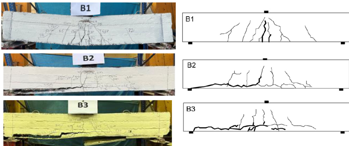
Fig. (9). Crack patterns of tested specimens in group one.
