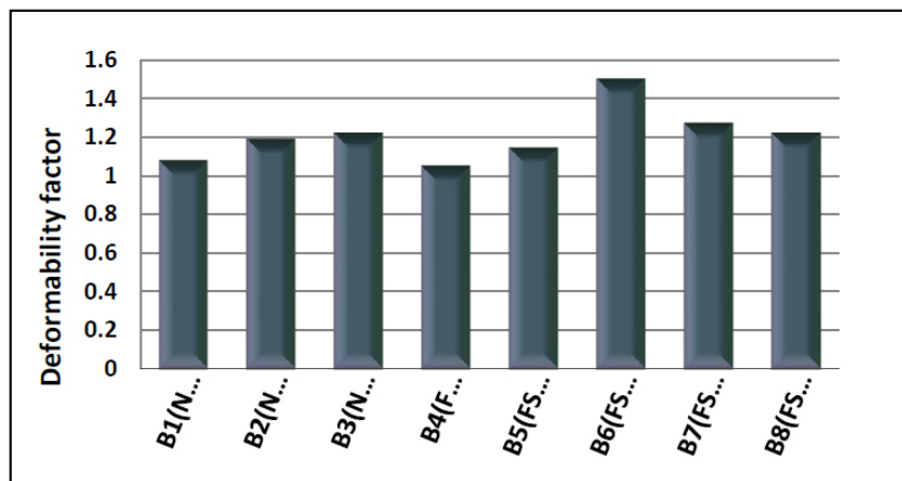
Fig. (25). Deformability factors for tested specimens.
