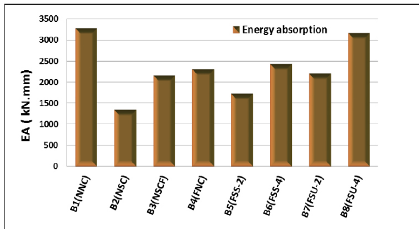
Fig. (23). Energy absorption for the tested specimens.
