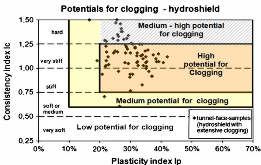
Fig. (4). Modified clogging diagram for slurry excavation machines [4].
