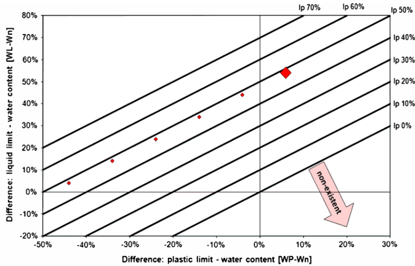
Fig. (7). The original shape of the new diagram with plastic index lines [4].
