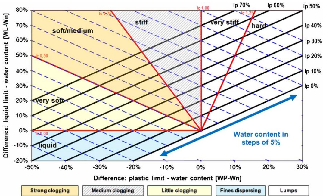
Fig. (10). General classification diagram for the critical consistency changes with respect to clogging [4].
