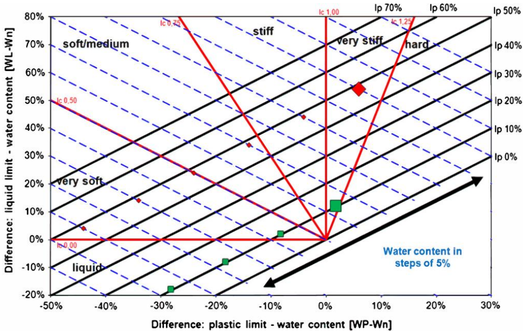
Fig. (9). Original shape of the new diagram with a scale to estimate the water content (the distance between two blue lines illustrates 5% of difference in terms of water content) [4].
