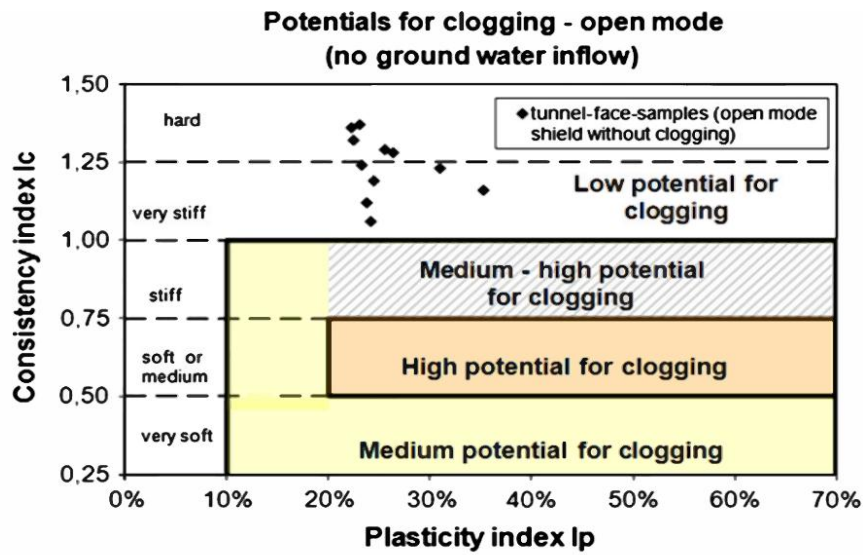
Fig. (5). Potential of clogging for open-mode machines without ground water inflow [4].
