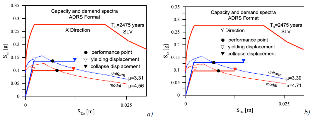
Fig. (17). Capacity and demand spectra in AD format: (a) X Direction; (b) Y Direction.
