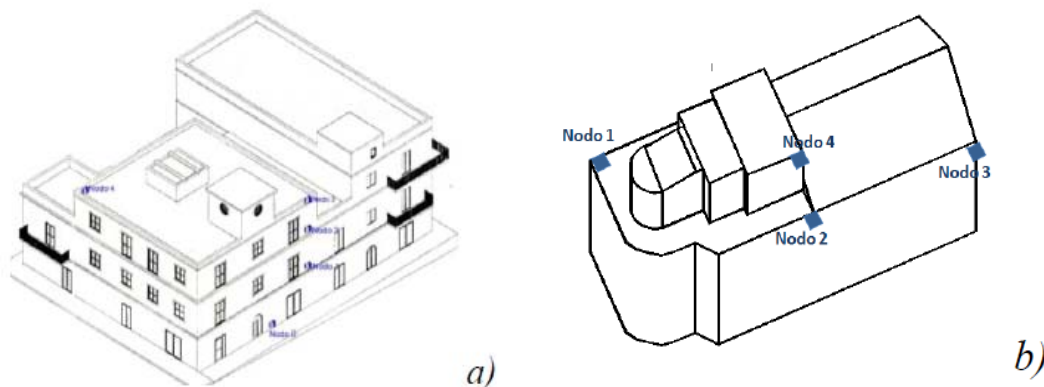
Fig. (11). Position of the acquisition nodes: (a) BT "A"; (b) BT "B".
