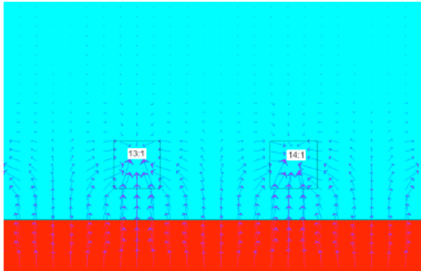
Fig. (9). The calculated airflow around air ducts No. 13:1 and No. 14:1 in the radon sub-slab suctioning system. For the calculation, the air permeability of the concrete was 0.018 \text{ g}/(\text{m h KPa}) . The pressure inside was 101\,323.24 \text{ Pa} and the pressure in the air ducts was 101\,320.00 \text{ Pa} . The air permeability of EPS was 0.0144 \text{ g}/(\text{m h KPa}) . Arrows show the airflow and the length of the arrows visualizes the relative volume of air flowing.
