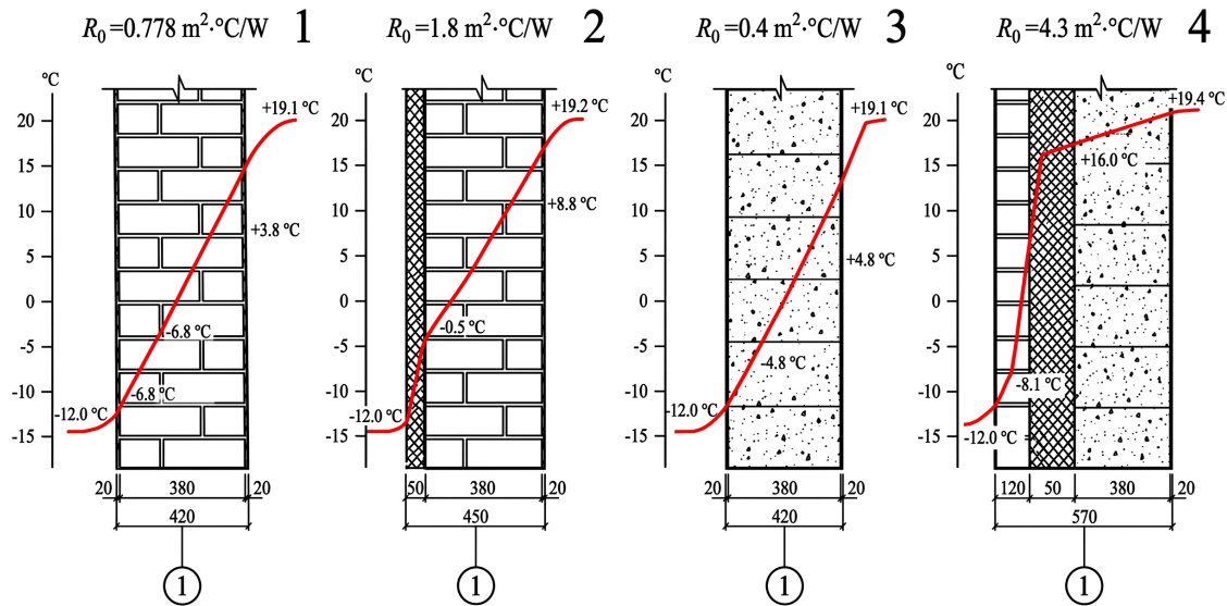
Fig. (2). Temperature distribution through external wall structures with different thermal resistance values: (1) fired brick wall, R_o = 0.778 \text{ m}^2\cdot\text{°C/W} ; (2) thermally protected brick wall, R_o = 1.8 \text{ m}^2\cdot\text{°C/W} ; (3) cinder block wall, R_o = 0.4 \text{ m}^2\cdot\text{°C/W} ; (4) multilayer insulated wall with reed insulation, R_o = 4.3 \text{ m}^2\cdot\text{°C/W} .
