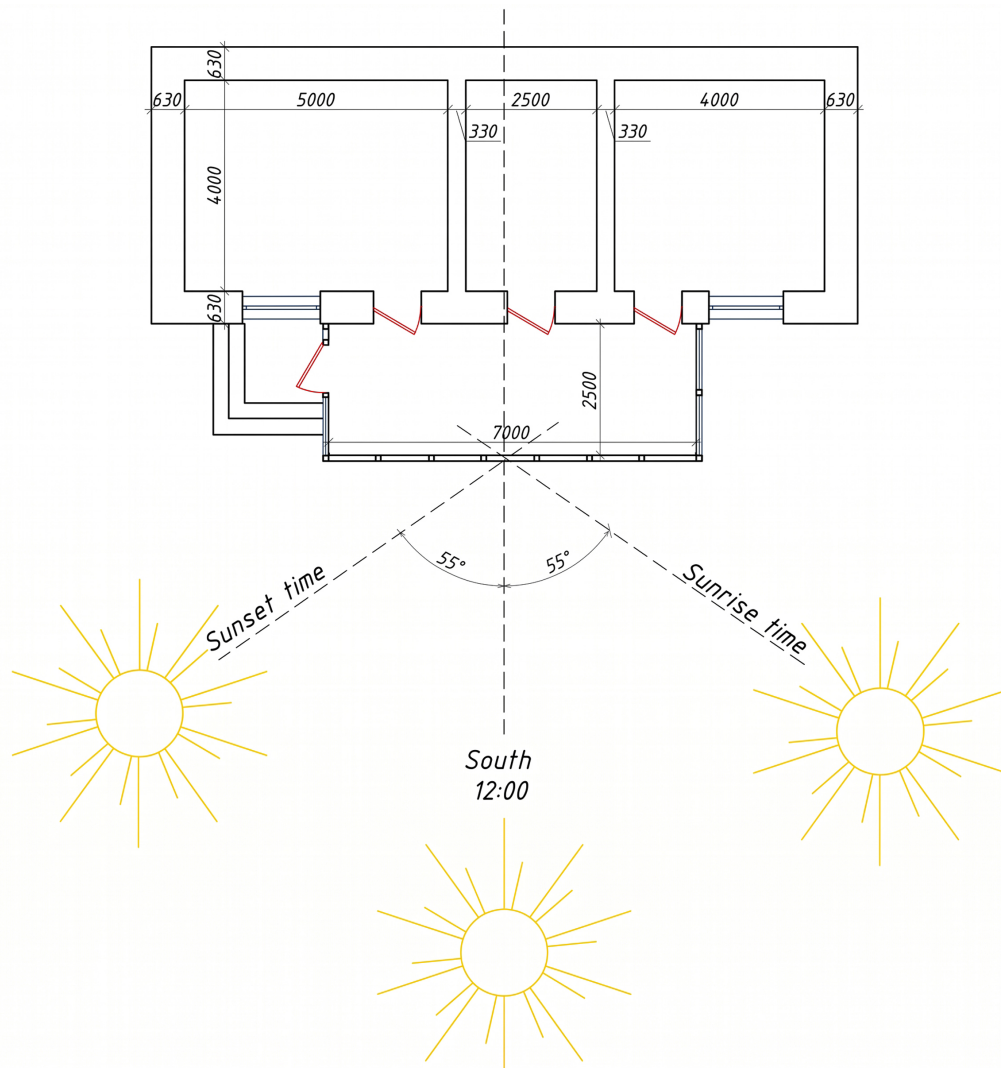
Fig. (1). Plan of the experimental residential building constructed from locally available materials.
