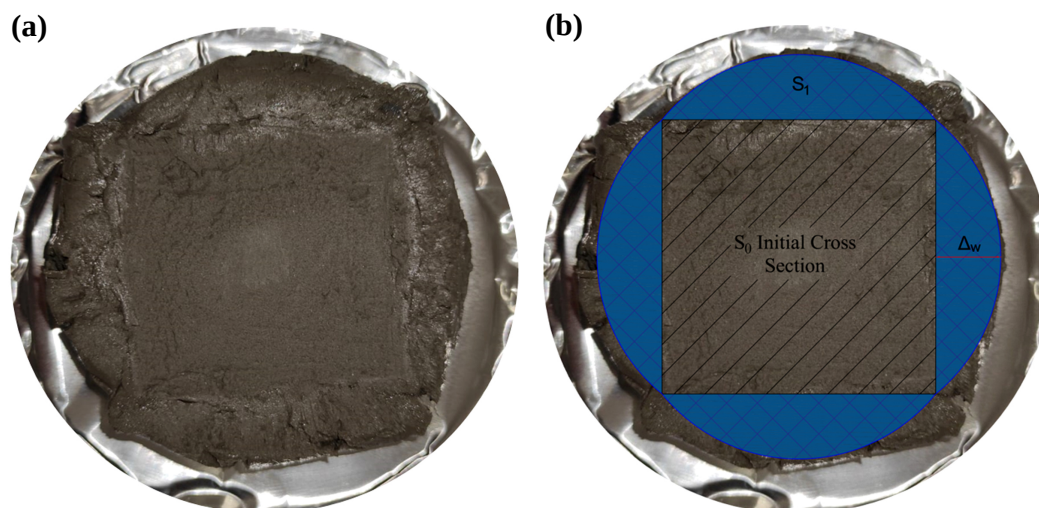
Fig. (10). Sample analysis after fresh UCT, (a) Deformed sample, (b) Cross-section analysis of material.
