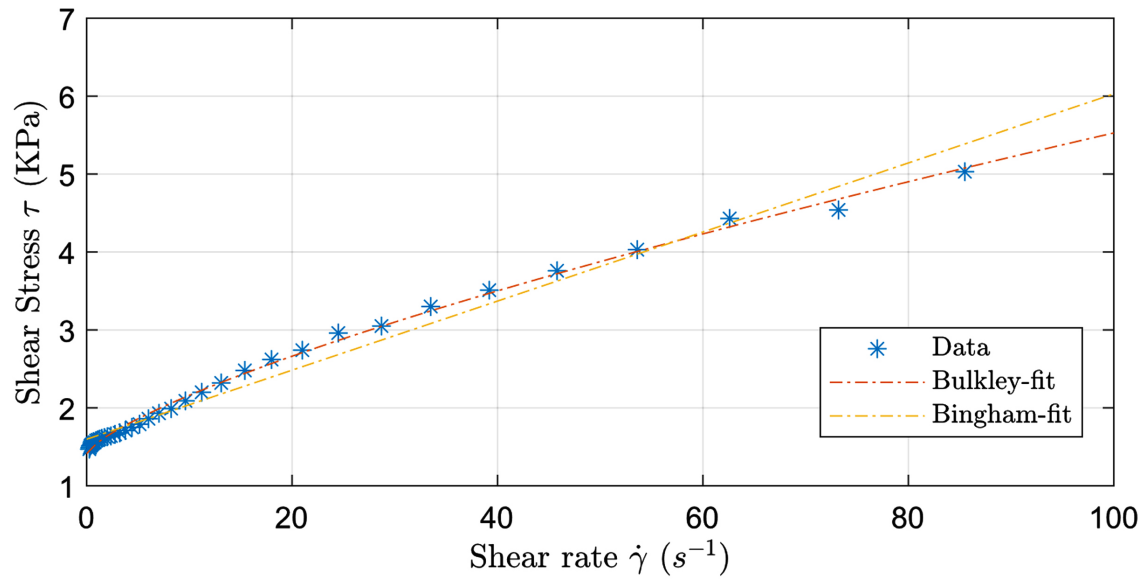
Fig. (14). Fresh paste rheological test. Reproduced from N. Rihani, F.Z. Oulakhir, N.C. Igwe, I. Akhrif, and M.E. Jai, "3D Clay Printing: A Taguchi approach to rheological properties and printability assessment", E3S Web Conf., vol. 601, 2025, under the permission of the Creative Commons Attribution License 4.0 [44].
