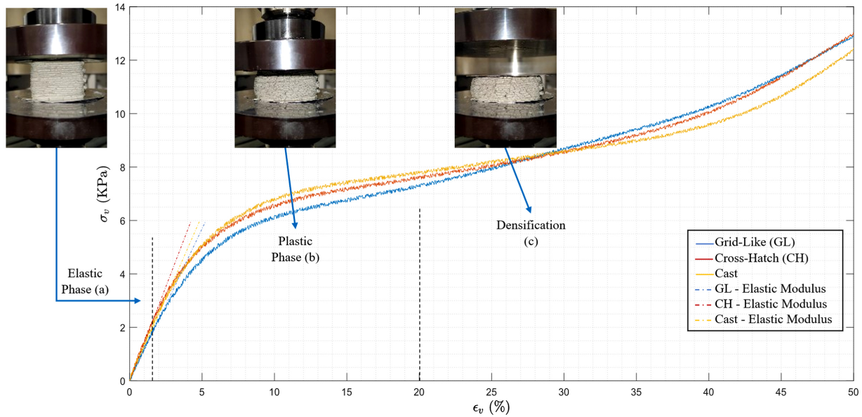
Fig. (9). Stress-strain curves from fresh UCT of clay specimens.
