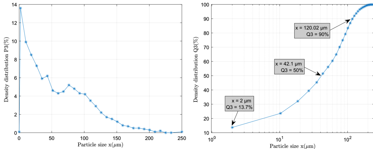
Fig. (6). Particle size and cumulative distributions.
