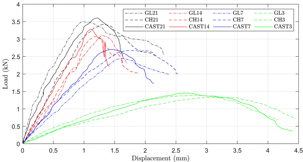
Fig. (16-A2). Load displacement curves for dry specimens.
