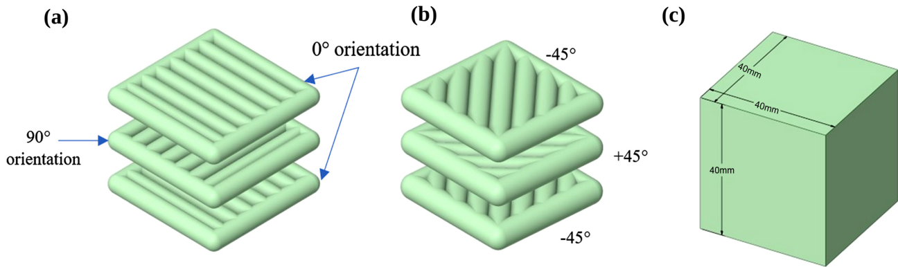
Fig. (1). 3D numerical model of the two infill strategies for 3D clay printing and molding of 40 mm cubes. (a) Grid-Like Infill (GL), (b) Diagonal Cross-Hatch Infill (CH), (c) Molded samples.
