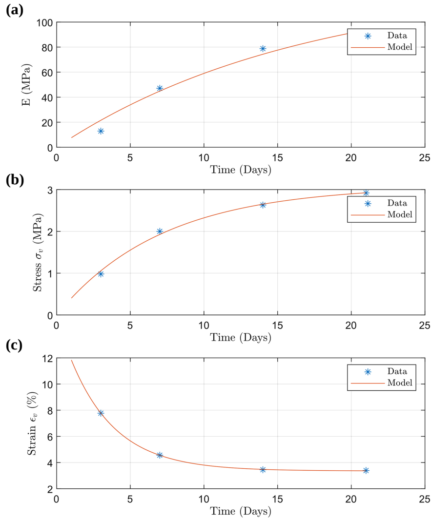
Fig. (12). Mean effect charts and the corresponding fitting. (a) mean young modulus, (b) mean vertical stresses, (c) mean vertical strains.
