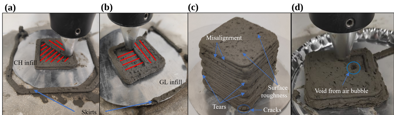
Fig. (7). 3D clay printing of samples with different infill strategies. (a) Cross-Hatch (CH) Infill, (b) Grid-Like (GL) Infill, (c) fully printed cubic sample with minor defect, (d) Major defect during deposition.
