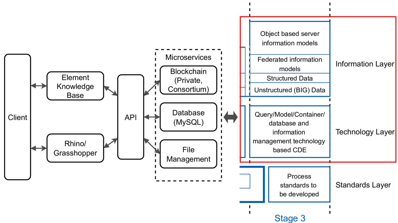
Fig. (4). The DISBS system architecture completes the environment of the ISO 19650-1 stage 3 technology layer.
