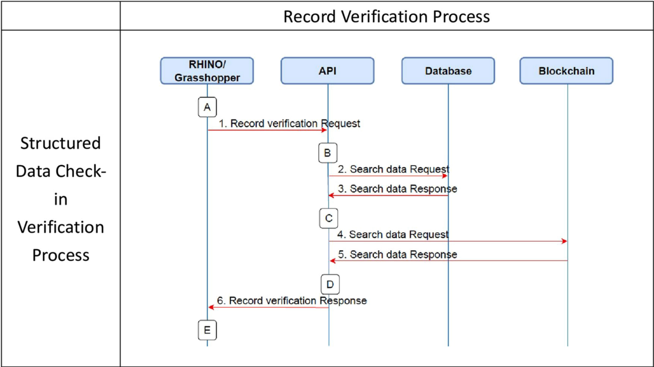
Fig. (9). Record verification process corresponding to the 19650-1 stage 3 technology layer.
