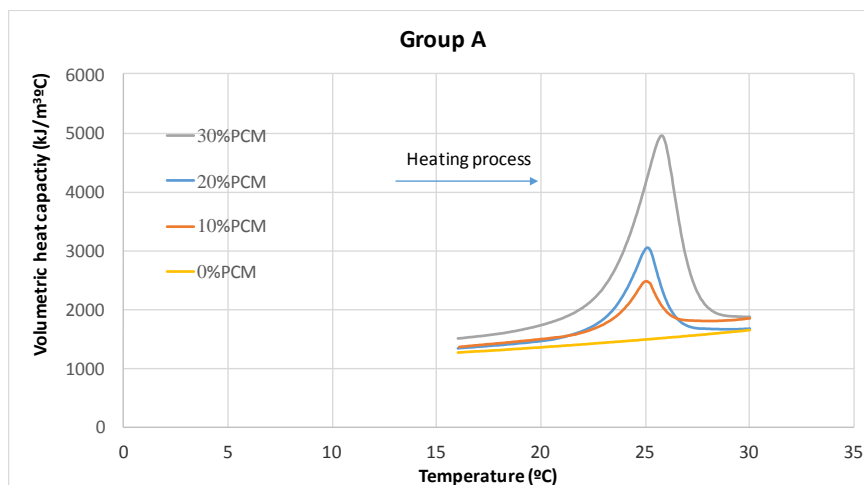
Fig. (9). Results for volumetric specific heat capacities of mortars at group A upon the heating process.
