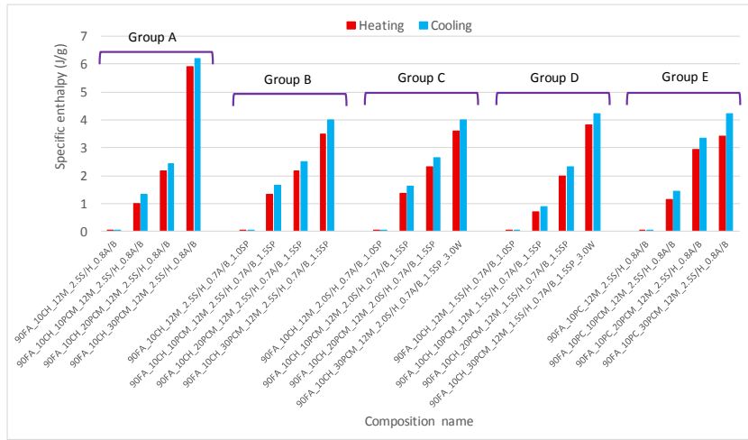
Fig. (11). Specific enthalpy values of the AACB mortars.
