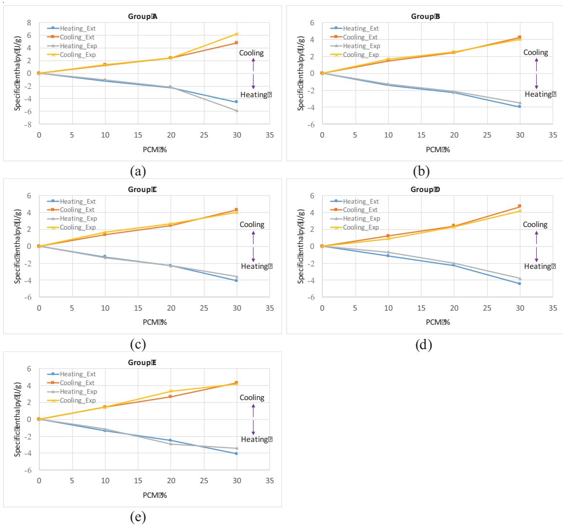
Fig. (12). Heat storage capacity of mortars for different groups: measured values (Exp) and extrapolated values (Ext).
