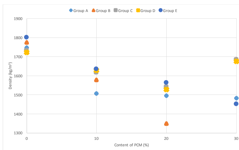
Fig. (4). Density versus PCM content for AACB mortars
