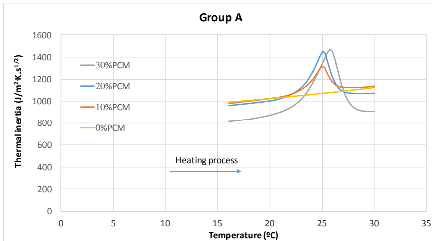
Fig. (10). Thermal inertia of mortars in function of temperature.
