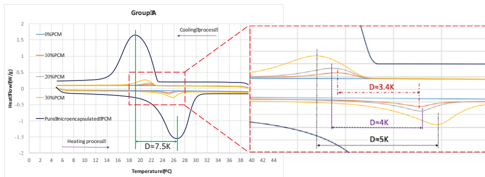
Fig. (8). Comparison between DSC curves for mortars in group A for a heating/cooling cycle at rate of 5°C/min, highlighting hysteretic behavior of mortars with PCM. “D” stands for the temperature difference between the peaks of heating and cooling processes.
