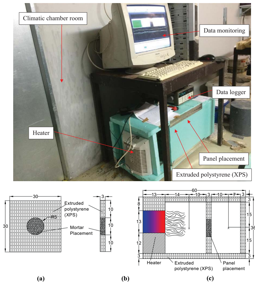
Fig. (3). Above: Photo of the prototype Below: Schematic representation of pilot prototype: (a) front view of the panel; (b) lateral view of the panel; (c) cross section of the test setup equipped with a heater together with placement of the panel inside the pilot prototype. Units: [cm].
