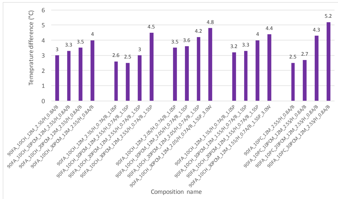
Fig. (14). Temperature differences between the maximum temperature and minimum temperature monitored at left and right side of the panel within prototype along tested time for all compositions.
