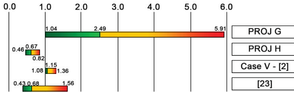
Fig. (15). Comparison of productivity (M³/hr/m²) in G and H and reference studies.
