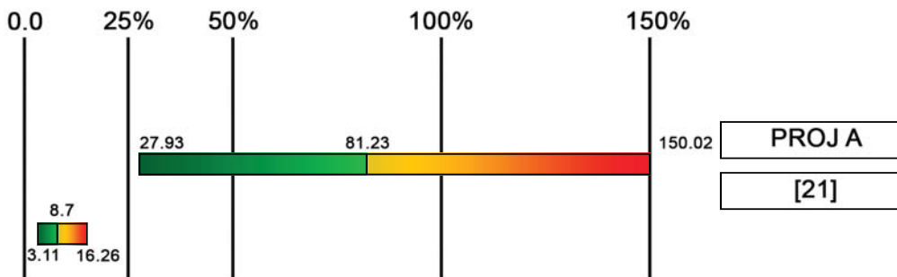
Fig. (7). Comparison of industrialized mortar losses (%) from project A and reference studies.
